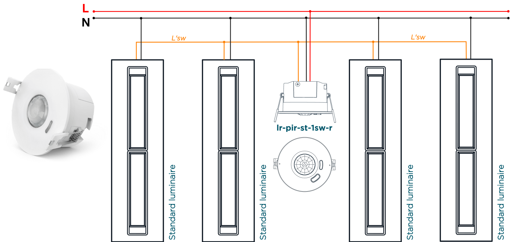
Example wiring of zencontrol standalone 240v smart PIR
