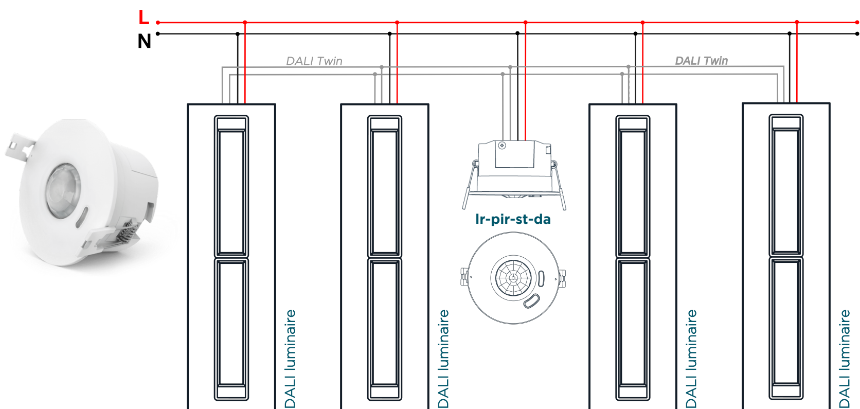
Example wiring of a zencontrol standalone DALI smart PIR
