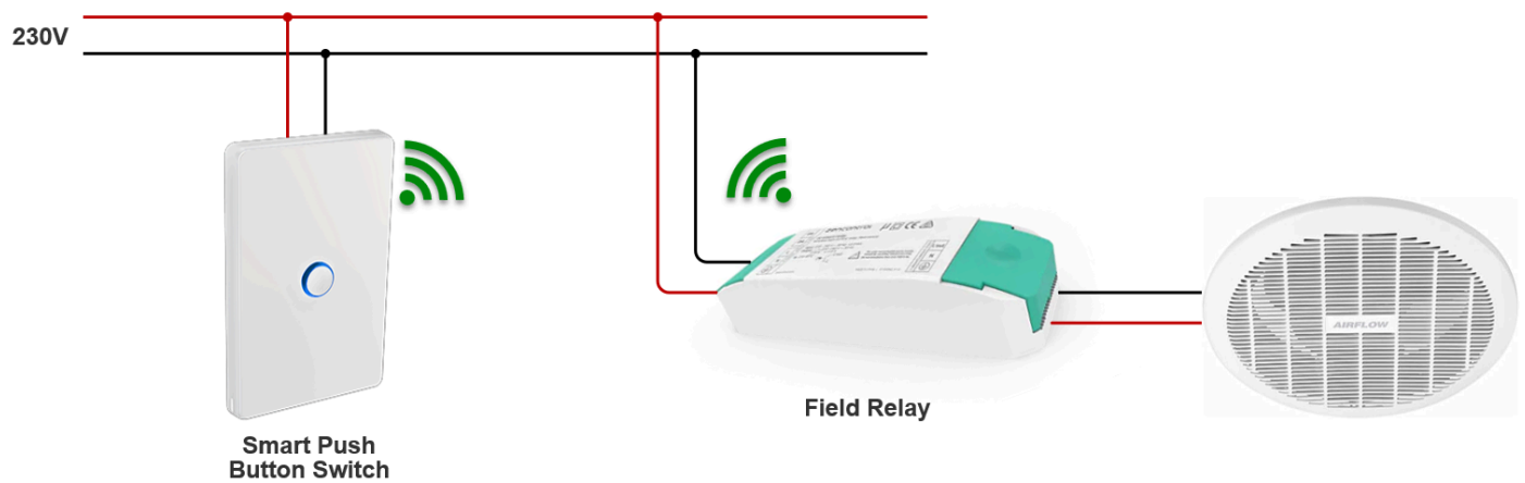
ReadyToGo Wireless Switch Kit Diagram
