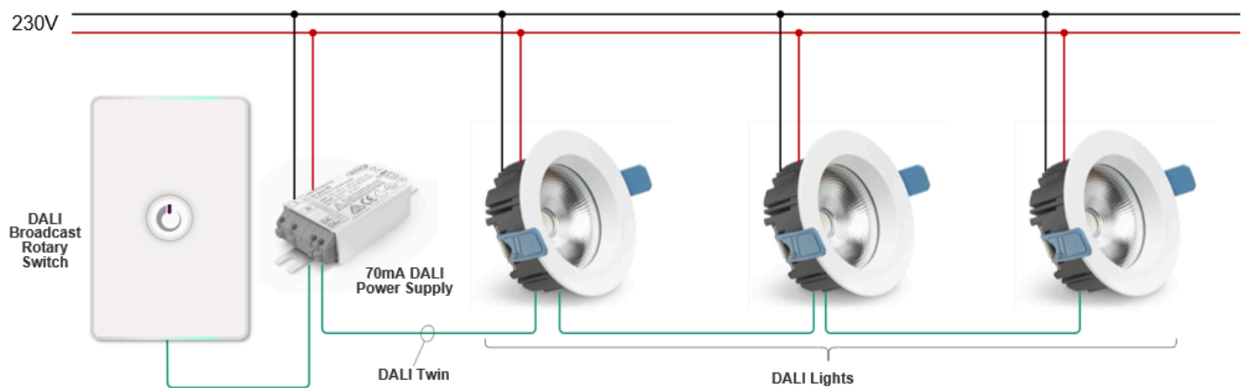
ReadyToGo DALI Broadcast Rotary Kit Wiring Diagram
