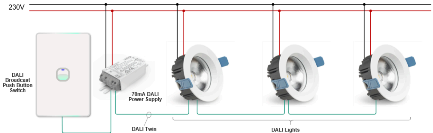
ReadyToGo DALI Broadcast Push Button Kit Wiring Diagram
